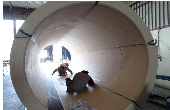
application of rubber lining layers
